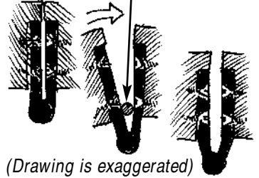
Use steel rod (like screwdriver) to bend open hinge
